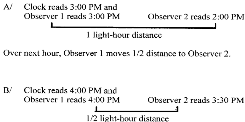
Figure 12.16 Clocks Moving Towards Each Other
