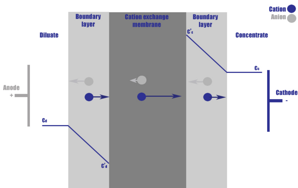
Figure 5: Concentration polarization
