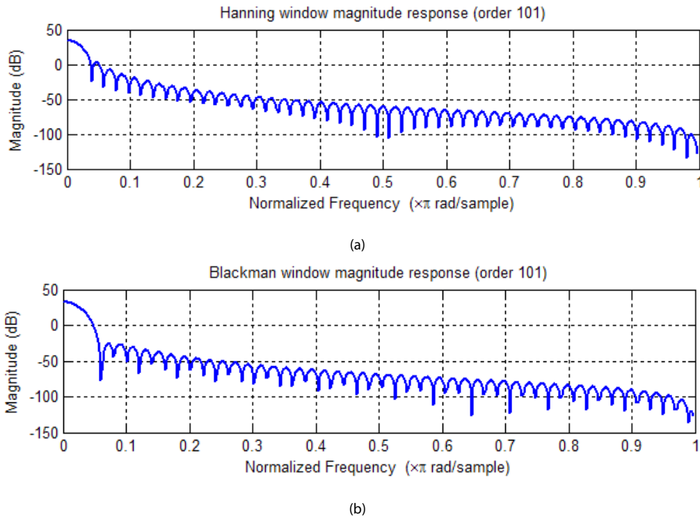
Figure 4.24: Window magnitude response (a) Hanning (b) Blackman.
